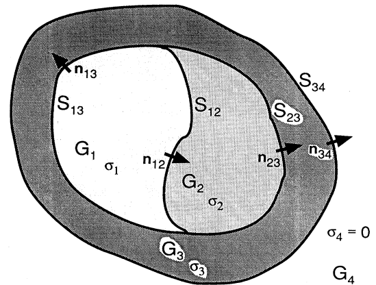
FIG. 18. Multicompartment conductivity model. Each region G_i has uniform conductivity \sigma_i . Unit vectors normal to the surfaces are denoted by \mathbf{n}_{ij} .
